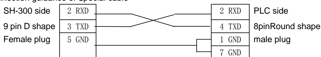
The picture for 8 pin Round shape Female plug
